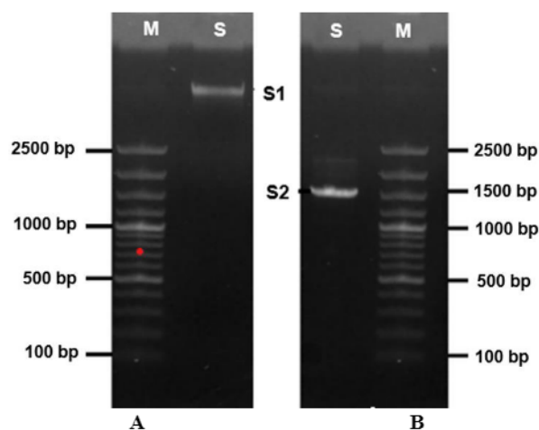
Figure 1. The electrophoresis results of DNA genome (A) and 16S rRNA gene (B) of Bacillus sp. BK7.1 on 1% agarose gel. Descriptions: M 100 bp DNA marker, S sample, S1 sample of DNA genome, S2 sample of 16SrRNA gene
