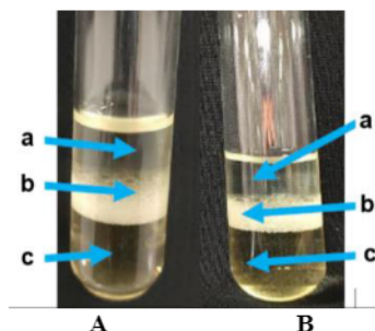
Figure 4. The emulsification activity of supernatant Bacillus subtilis BK7.1 on the kerosene substrate. A. 1 hour of exposure, B. 24 hours of exposure. a. kerosene, b. emulsion, c. isolate
