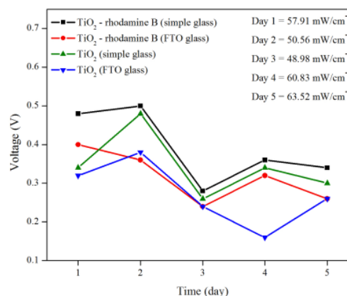
Fig. 6. Voltage vs time curve.
