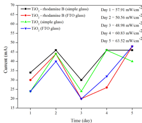
Fig. 5. Current vs time curve.
