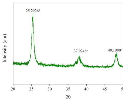
Fig. 3. The diffractogram of \text{TiO}_2 thin layer deposited on a simple glass plate.
