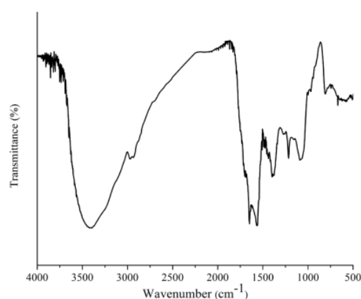
Fig. 5. FTIR Spectrum of FC300.
