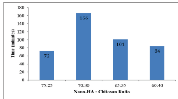
Fig. 2. The Setting time test results of IBS
