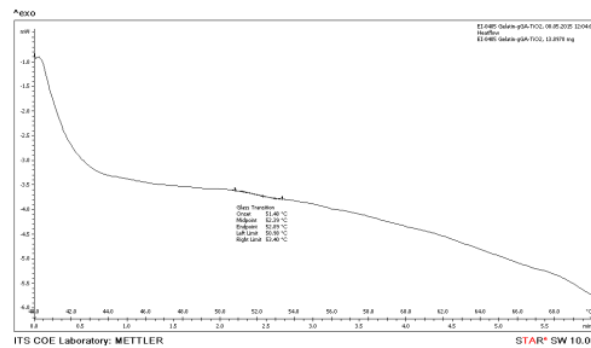
Figure 7. DSC thermogram gelatine composite-GA- \text{TiO}_2
