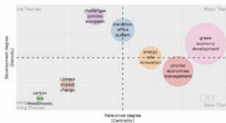
Figure 8: Thematic Map
