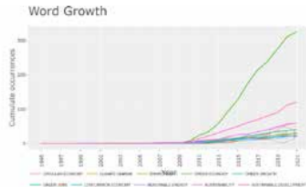
Figure 5: Word Dynamic
