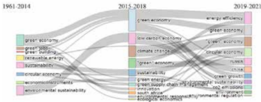
Figure 9: Thematic Evolution
