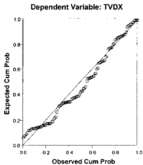
Normal P-P Plot of Regression Standardized Residual - 2009
