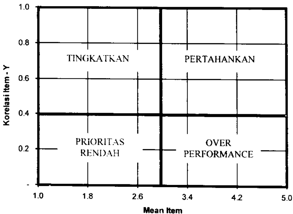
Gambar 4.1 Analisis Kuadran
