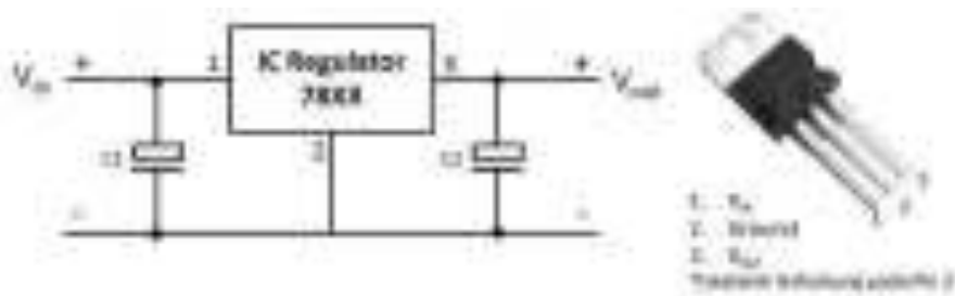
Gambar 2.4 Regulator
