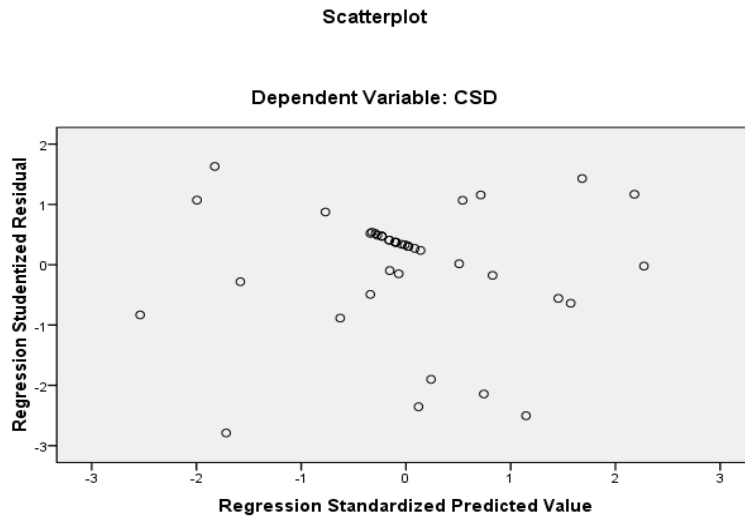
Gambar 1 Scatterplot
