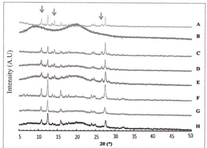
Figure 4: X-ray diffractograms of QC (A), hydroxypropyl methyl cellulose (B), physical mixture 1:1 (C), physical mixture 1:2 (D), physical mixture 1:3 (E), solid dispersion 1:1 (F), solid dispersion 1:2 (G), and solid dispersion 1:3 (H)
