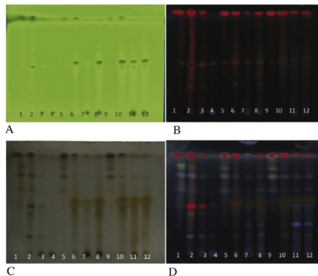
Figure 2. TLC analysis of extracts of A. altilis , A. heterophyllum and A. camansi .
