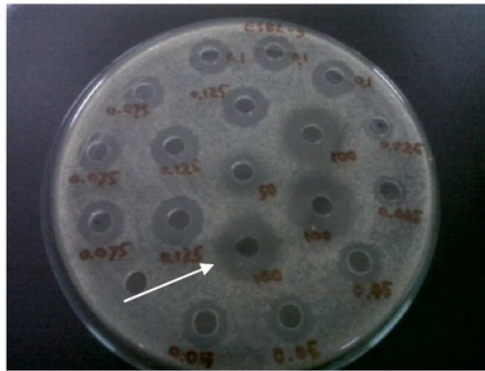
Figure 2. Inhibition activity of concentrate of free cells probiotic fermentation broth (100), meropenem at concentration of 0.05, 0.075, 0.10, 0.125 ppm against ESBL growth on the nutrient agar medium
