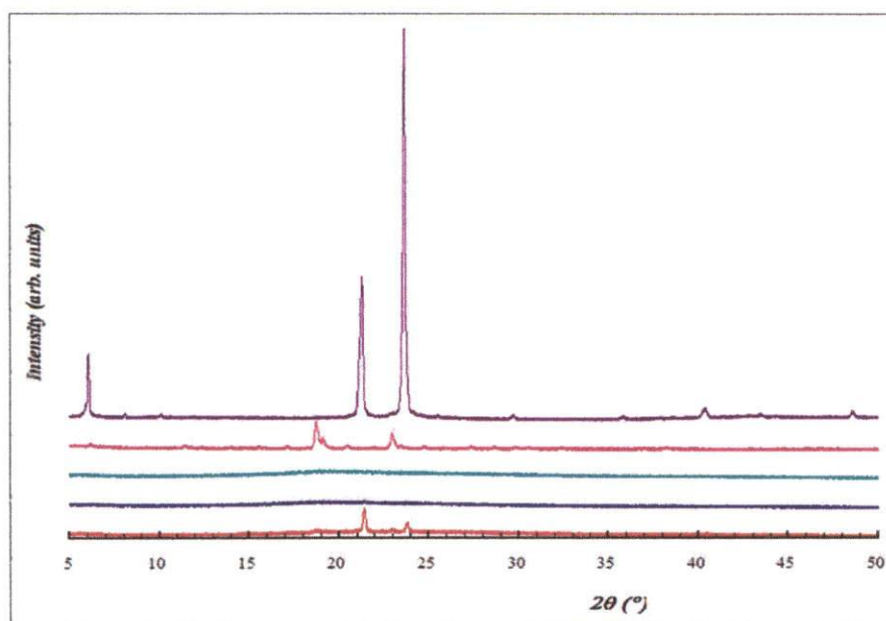
Fig. 7: The examination result of X-ray diffraction. (a) F3, (b) F2, (c) F1, (d) coenzyme Q10, (e) cetyl palmitate
