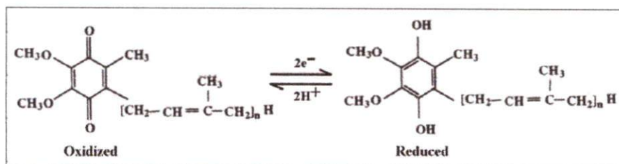
Fig. 1: Oxidized and reduced forms of coenzyme Q: In humans, the number of isoprene units (n) is 10
