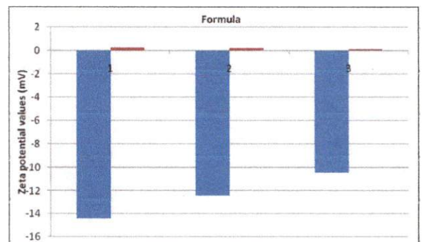
Fig. 6: The histogram of some nanostructured lipid carrier formulas average zeta potential in aqueous media using Malvern Instrument®
