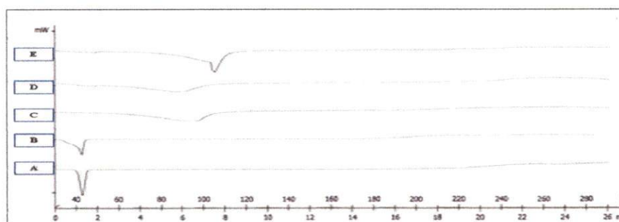
Fig. 8: The examination result of differential scanning calorimetry, (a) coenzyme Q10; (b) cetyl palmitate; (c) F1; (d) F2; (e) F3
