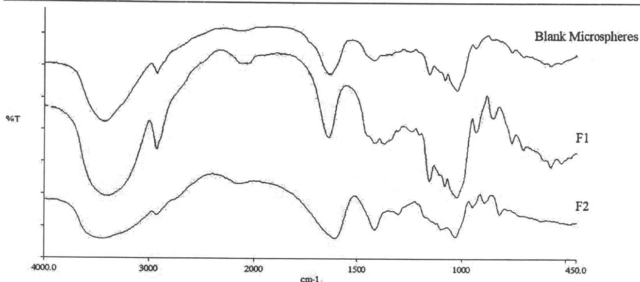
Figure 2. IR spectrum of glutathione-alginate microspheres.
