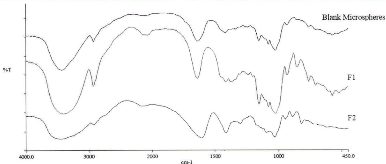
Figure 2. IR spectrum of glutathione-alginate microspheres.
