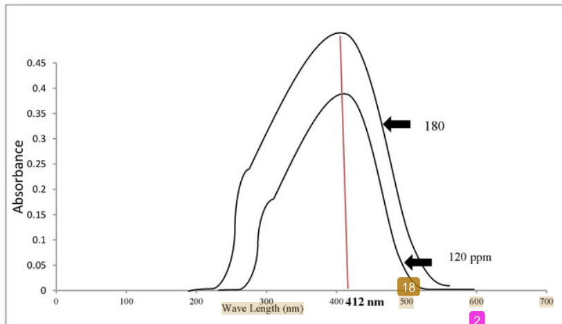
Figure 1: Absorption Profile of Glutathione Standard Solution 120 ppm, and 180 ppm in 0.01 M phosphate buffer solution pH 6.0 ± 0.05.
