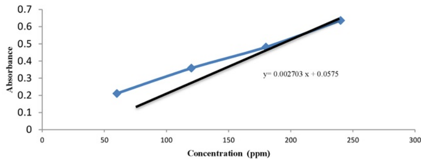
Figure 2: Glutathione in Phosphate buffer pH 6.00 ± 0.05.
