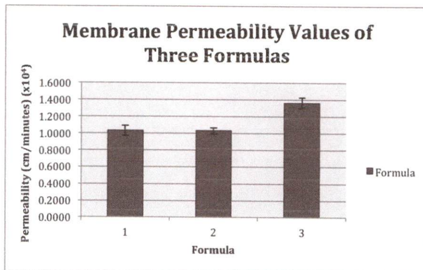
Figure 4. Membrane Permeability toward Diclofenac Sodium.
