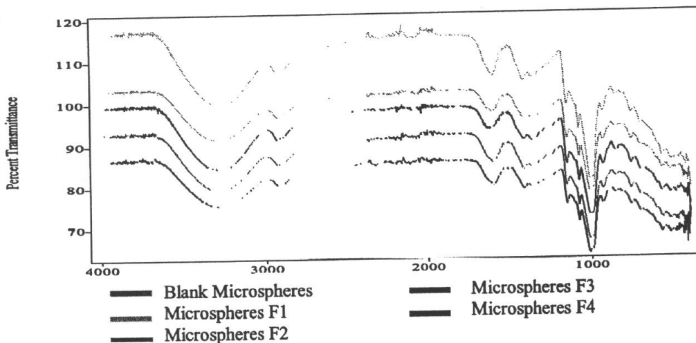
Figure 1. The overlay result of IR spectrum examination of metformin-alginate microspheres with the ratio of metformin amount
