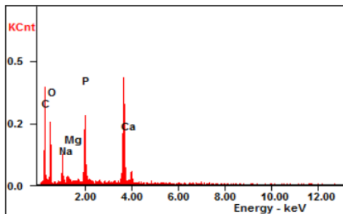
Figure 3. SEM-EDX spectrum of scaffolds BHA-GEL-K
