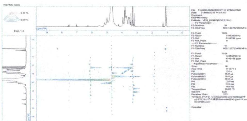
Fig.6. ROESY spectrum of solution containing the 1:1 molar ratio of EPMS-HP- \beta -CD inclusion complex (D 2 O).
