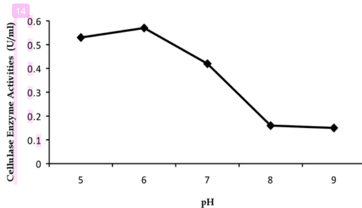
Figure 2. The pattern of relationship between pH and the cellulase enzyme activities.
