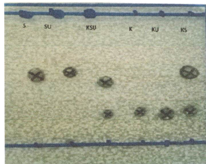
Figure 1. The retardation factor (R f ) of streptomycin sulfate (S) and kanamycin sulfate (K) in shrimp (U) for the determination of resolution (R s ) value
