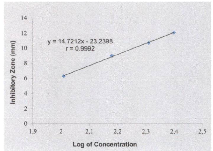
Figure 2. Linear regression of streptomycin sulfate analyzed using contact TLC-bioautography
