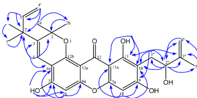
Figure 2. Selected HMBC correlation for 5,9,11-trihydroxy-10-(2''-hydroxy-3''-methylbut-3''-en-1-yl)-2,2-dimethyl-3-(2'-methylbut-3'-en-2'-yl)-2H,12H-pyrano[2,3-a]xanthen-12-one.
