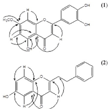
Fig. 2. HMBC correlation of compound 1 and compound 2 .
