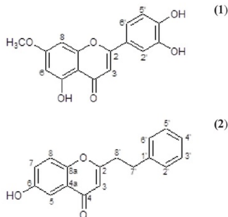
Fig. 1. Structure of isolated compounds.
