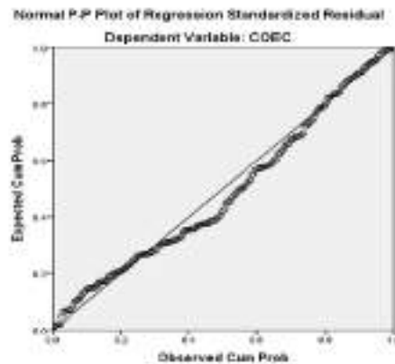
Figure 2. Graph of Normality P-P Plot Equation 2
