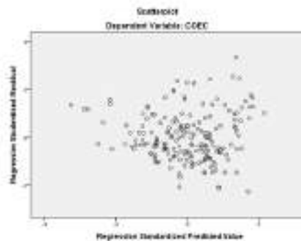
Figure 3. Heteroscedasticity test of equation 1
