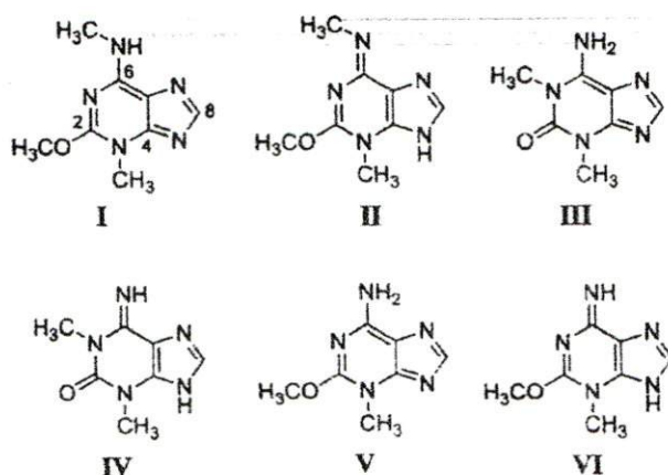
Scheme 1 The two tautomeric forms ((I) and (II)) of N6-methyl mucronatine and the equivalent tautomeric forms for 1,3-dimethylisoguanine ((III) and (IV)) and for mucronatine ((V) and (VI))
