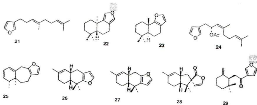
Fig. 2 Representative sesquiterpene metabolites isolated from Hypselodoris mollusks.
