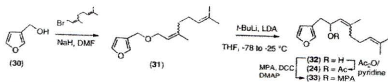
Scheme 1 Synthetic route to dendrolasin-5-acetate ( 24 ).
