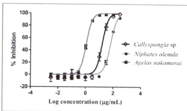
Fig. 1. Dose-dependent response of selected marine sponges to the inhibition of acetylcholinesterase. Data presented as mean \pm standard deviation of three independent experiments.
