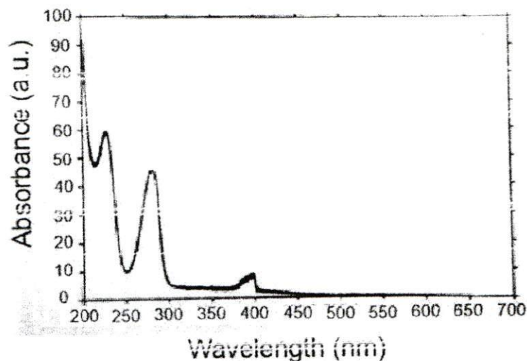
Figure 2. UV-visible absorption spectra of fraction a using TLC-densitometry.
