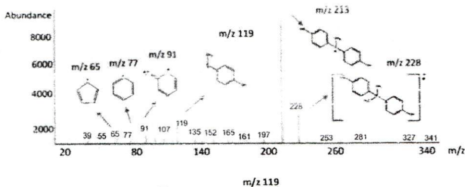
Figure 4. EI-MS of peak 1 of fraction a.
