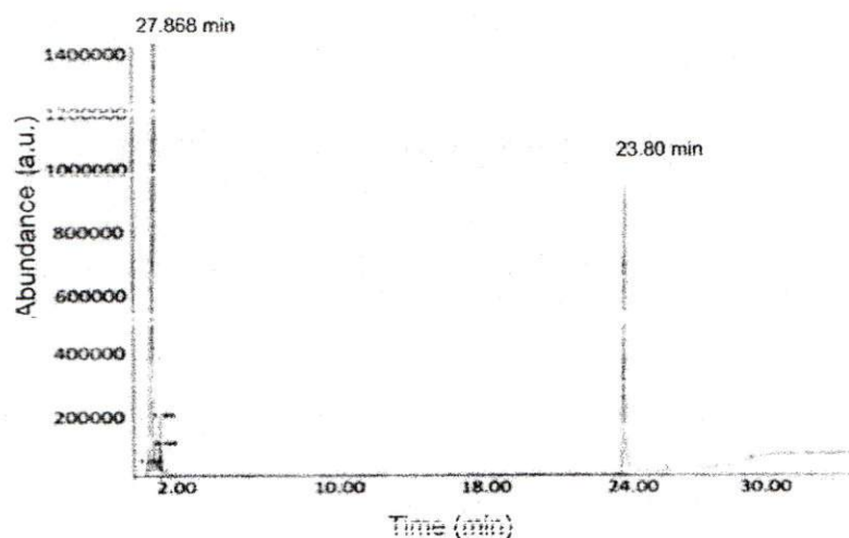
Figure 3. Total Ion Chromatogram of fraction a
