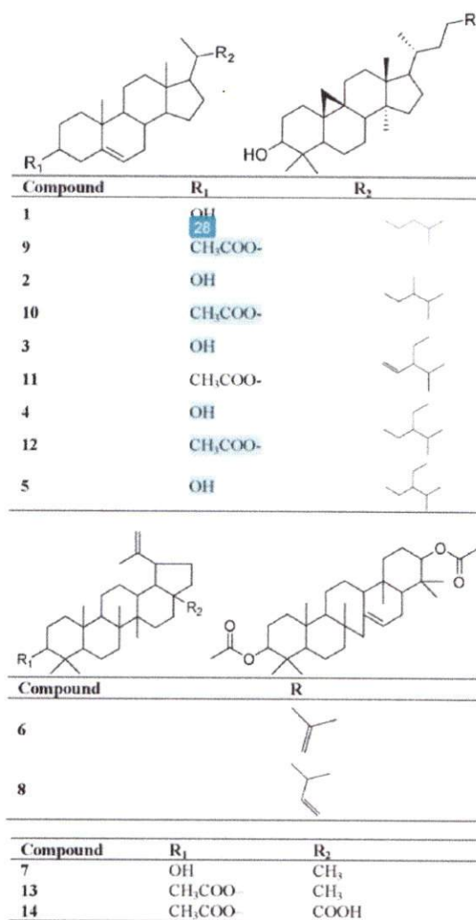
Figure 7. Structures of Identified Sterols and Triterpenes
