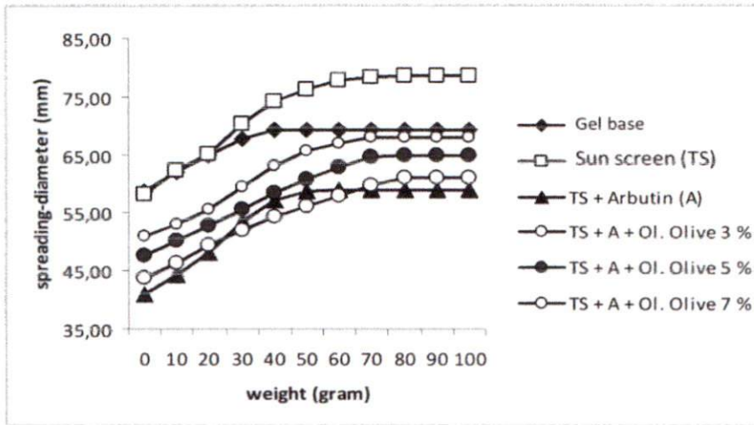
Figure 1. Spreading capability of sunscreen.
