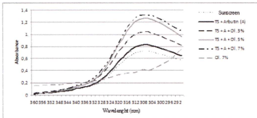
Figure 2. Absorption spectrum of sunscreen.
