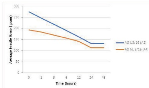
Figure 4 Force degradation trend for 3/16 inch AO latex and nonlatex elastics over time.
