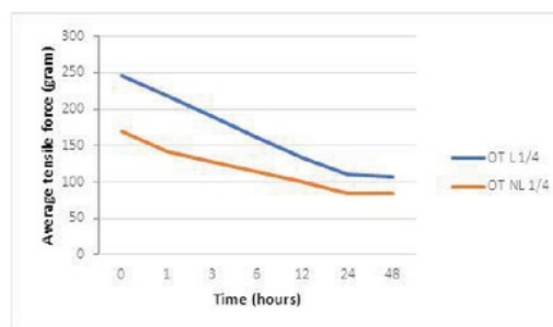
Figure 3 Force degradation trend for 1/4 inch OT latex and nonlatex elastics over time.
