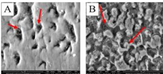
Figure 6. Microporosity of enamel from SEM result with 5000x magnification, the arrows indicate microporosity: A. After self-etching primer application. B. after phosphoric acid 37% application.
