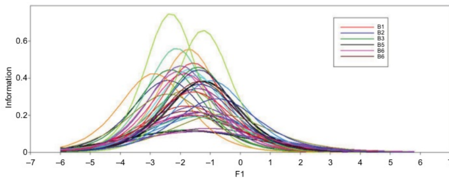
Figure 5 IIF values of subset 2. Abbreviation: IIF, item information function.
