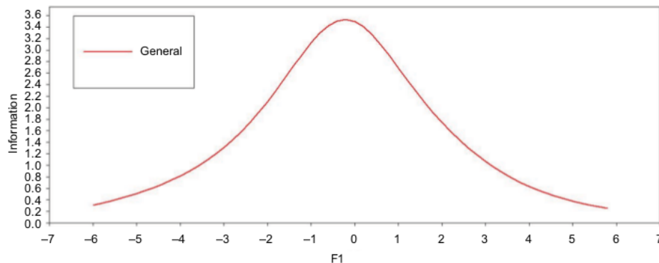
Figure 3 TIF values of subset 1.
