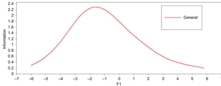
Figure 9 TIF values of subset 3.
