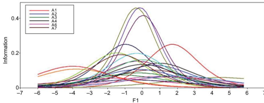
Figure 2 IIF values of subset 1.
