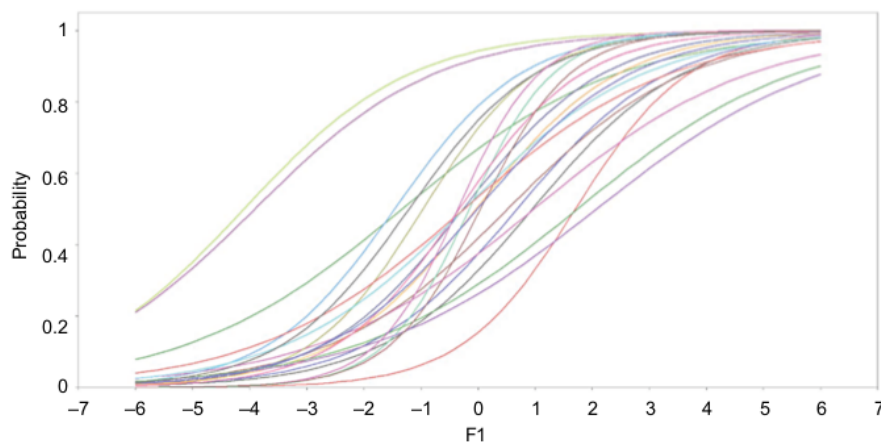
Figure 1 ICCs of subset 1. Abbreviation: ICC, item characteristic curve.
