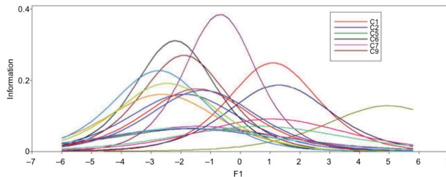
Figure 8 IIF values of subset 3.
