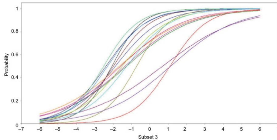
Figure 7 ICCs of subset 3.
