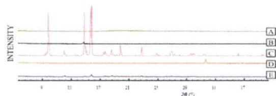
Figure 3. X-ray diffractogram of (A) carboxymethyl chitosan, (B) \text{CaCl}_2 , (C) andrographolide (D) crosslinked andrographolide-chitosan particles, and (E) physical mixture of andrographolide-chitosan
