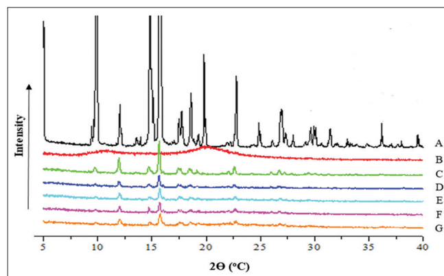
Figure 4: X-ray diffractograms of (a) andrographolide, (b) chitosan, and andrographolide-chitosan solid dispersion system with various drug-polymer ratio: (c) 1:1, (d) 1:2, (e) 1:3 (f) 1:4, and (g) 1:5
