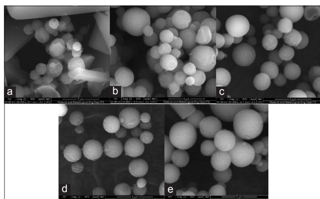
Figure 1: Scanning electron microscopy micrograph of andrographolide-chitosan solid dispersion system with various drug-polymer ratio (a) 1:1, (b) 1:2, (c) 1:3, (d) 1:4, and (e) 1:5 with \times 20000 magnification
