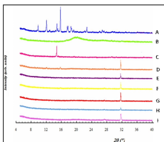
Figure 5. X-ray diffractogram of: (A) DTLF; (B) CMChi; (C) \text{CaCl}_2 , and nanoparticulate of CMChi- \text{CaCl}_2 -DTLF of formula: F3 (D), F4 (F), F5 (F). (E), (G), (I): Nanoparticulate system of CMChi- \text{CaCl}_2 without DTLF:
