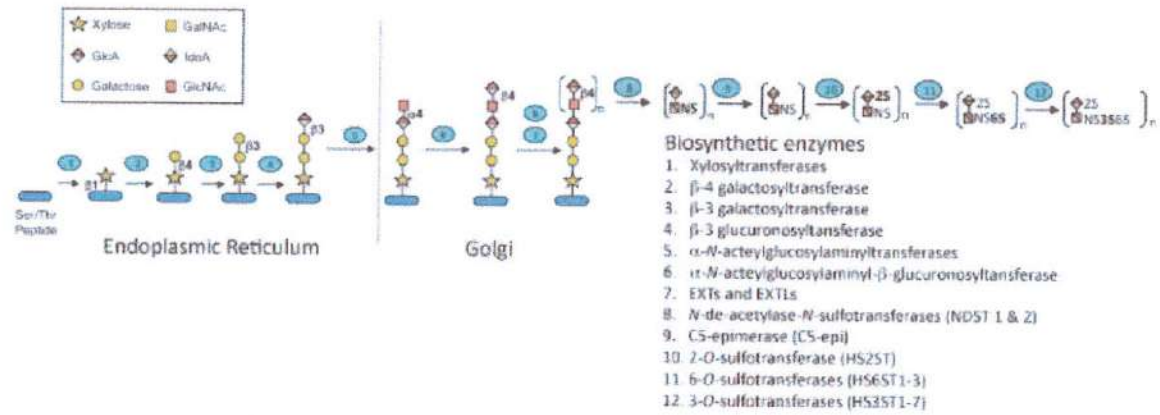
Figure 2. Heparin biosynthesis.
