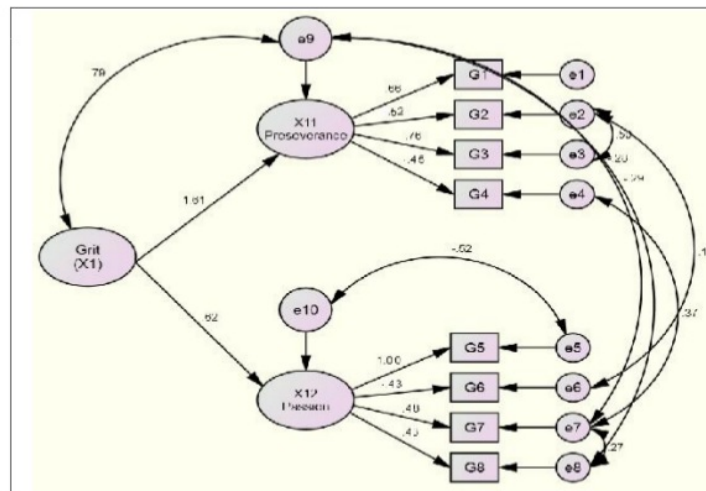
Figure 2. Second-order Model CFA-2 Model for Grit construct
