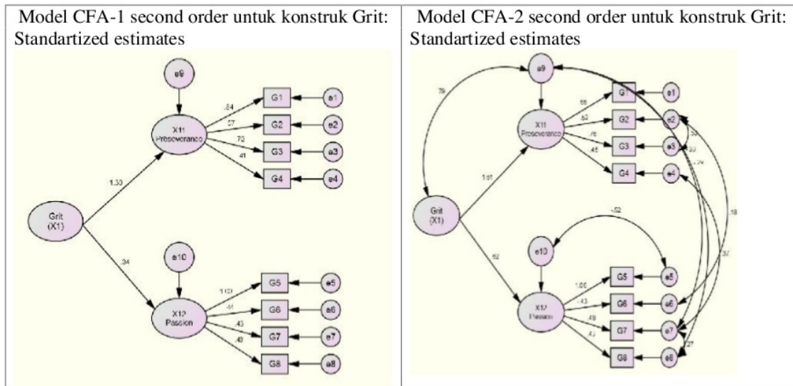
Figure 1. Model CFA 1 and CFA 2
