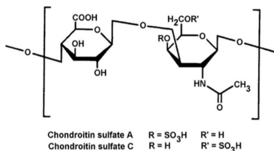
Figure 1: Structures of chondroitin sulphate.
