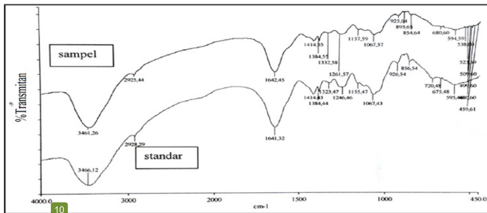
Figure 2: Overlay spectra of CS standard and CS from chicken shank
