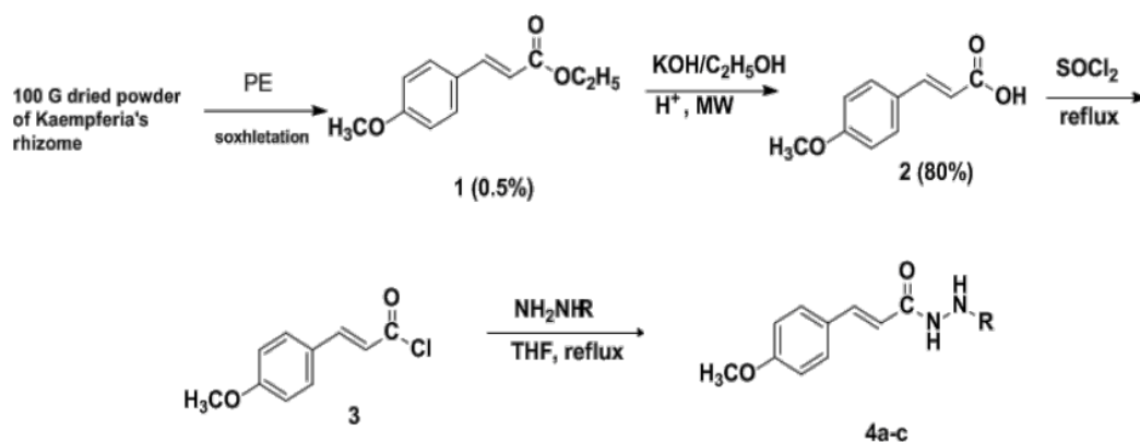
Figure 1: Synthesis of p -methoxycinnamoyl hydrazides.
