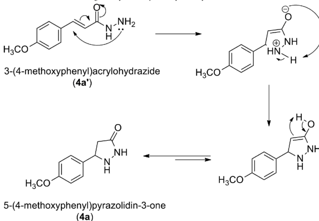
Figure 2: Cyclization of 3-(4-methoxyphenyl)acrylohydrazide.
