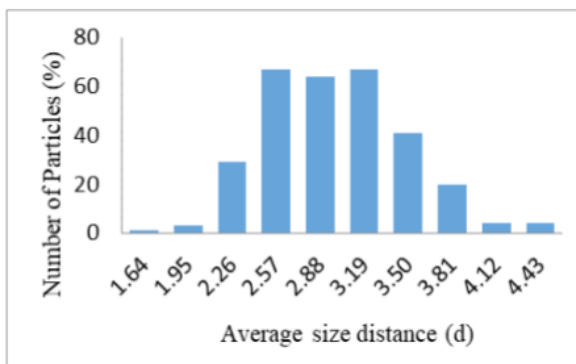
Figure 4: Particle size distribution of gentamicin sulphate microspheres.
