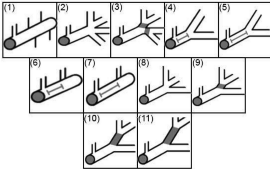
Fig. 1. The 11 different branching patterns of MCAs.
