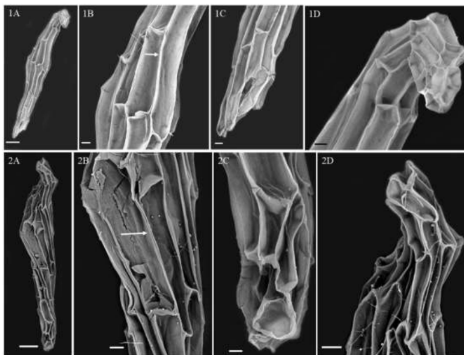
Figure 5. SEM photographs. 1. Paph. baccanum . 2. Paph. kolopakingii . A. Fusiform seed shape, B. Testa cells of the medial (1B. arrow indicate the testa cell walls are thin, 2B. arrow indicates the cell walls were flat), C. Basal pole, D. Apical pole. Scale bars: A=80 \mu\text{m} , B-D = 20 \mu\text{m} .
