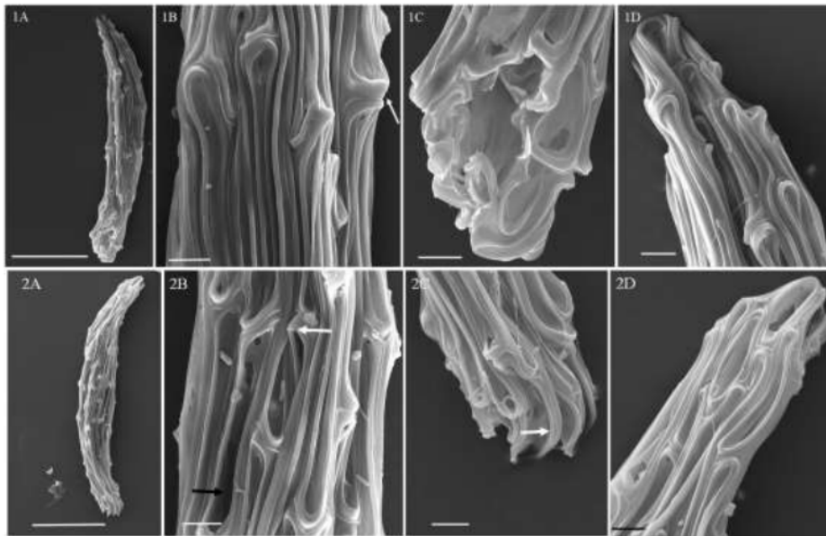
Figure 3. SEM photographs. 1. Phal. bellina , 2. Phal. gigantea , A. Seed shape, B. Testa cells of the medial (1B. arrow indicate cells are rounded and slightly raised, 2B white arrow indicates the testa cell are curved and raised at the end of two testa cells, black arrow indicates ridge with deep groove) , C. Basal pole (2C. arrow indicate the end testa cells at the basal pole had appendage with point of the end), D. Apical pole. Scale bars: A=100 \mu m, B-D=10 \mu m.
