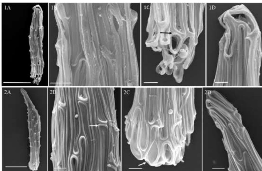
Figure 4. SEM photographs. 1. Phal. tetraspis . 2. Phal. venosa . A. seed shape, B. Testa cells of the medial (2B. arrow indicates the testa cell walls are raised at the end of the meeting between two cells) , C. Basal pole (1C. black arrow indicates the testa cell become wider, rounder, and rose up, 2C. arrow indicates the testa cells at the end of basal pole were widened and rounded), D. Apical pole. Scale bars: A=100 \mu\text{m} ; B-D = 10 \mu\text{m} .
