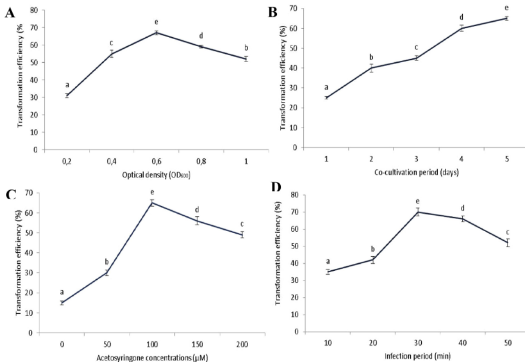
Fig. 3. Effects of various factors affecting transformation efficiency of D. lasianthera . A bacterial density, B co-cultivation period, C acetosyringone concentrations, D infection period.
