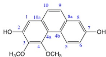
Fig. 2. Chemical structure of nudol ( 2 ).
