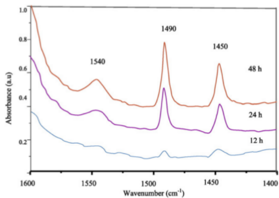
Fig. 3. Pyridine-FTIR spectra of amorphous mesoporous aluminosilicates synthesized directly from kaolin after adsorption of pyridine and evacuation at 150 ^{\circ}\text{C} for 3 h.
