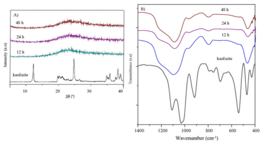
37 Fig. 1. A) XRD pattern and B) FTIR spectra of the synthesized amorphous mesoporous aluminosilicates at 12, 24 and 48 h.
