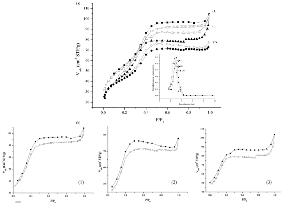
Fig. 4. N_2 adsorption/desorption isotherms (a) and hysteresis loop (b) of the samples at different hydrothermal temperature and time: 393 K, 11 h (1); 393 K, 24 h (2) and 393 K, 48 h (3)
