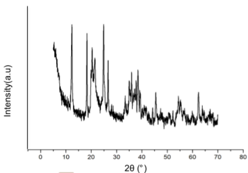
Fig. 2 XRD pattern of red mud.
